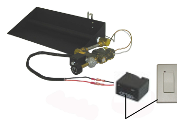
Battery Powered Wireless Wall Switch (WS-S6V-LTST)
