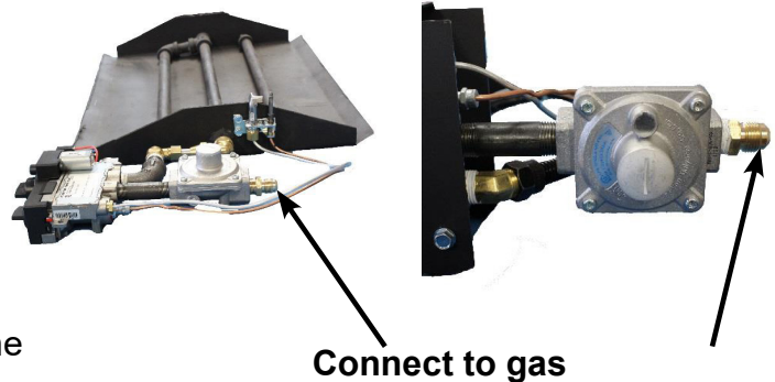
BURNER MOUNTED
