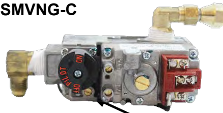
Pilot Adjustment Screw
